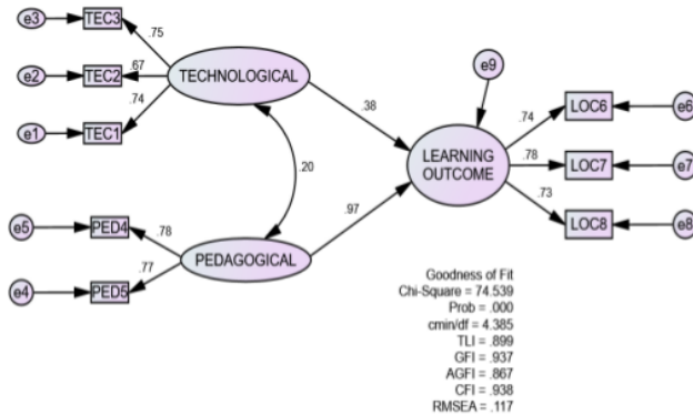
Figure 2. Model Goodness of Fit (GOF)
